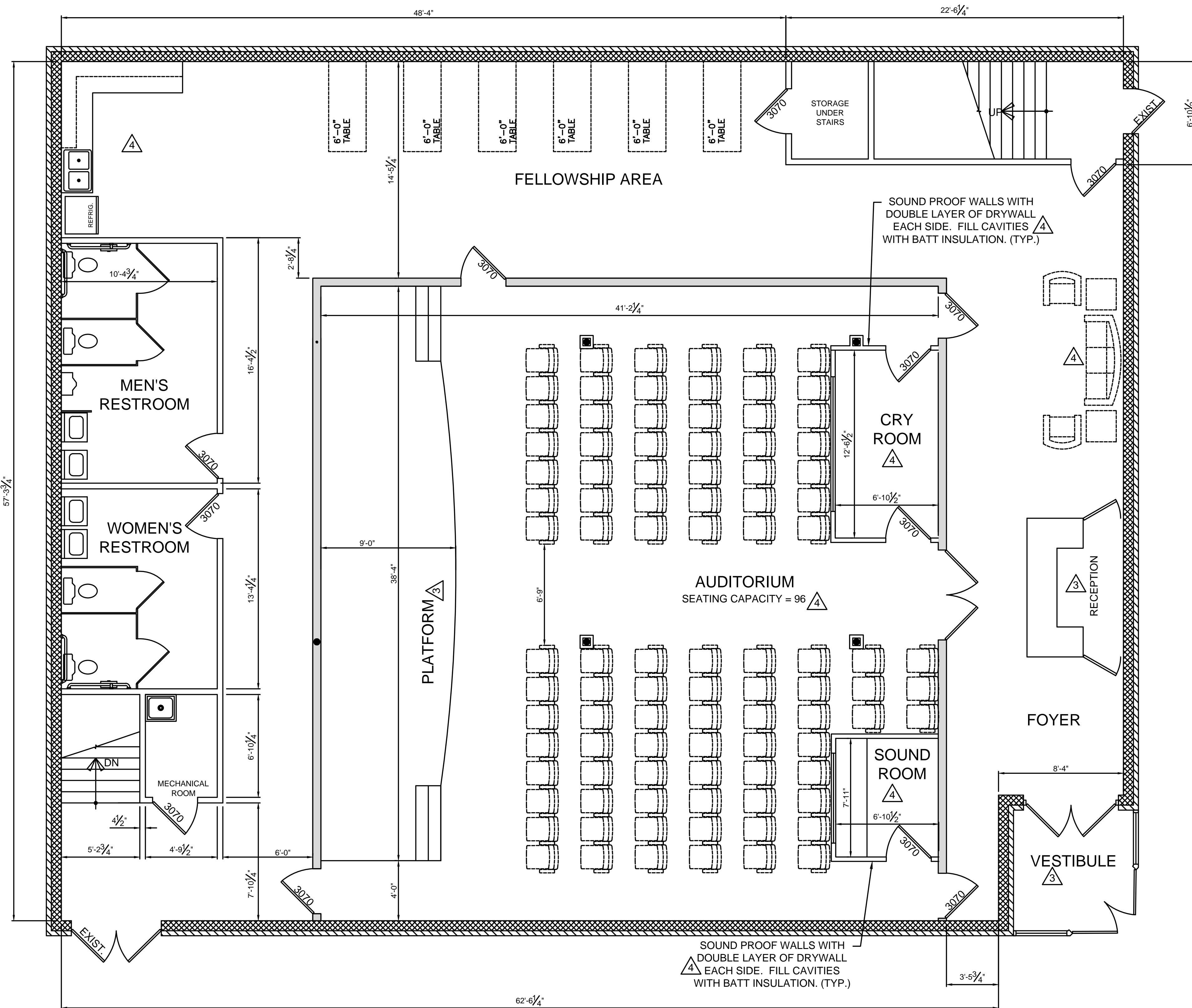
FLOOR PLAN - PHASE 1 3 / 4 SCALE: 1/4" = 1'-0"
